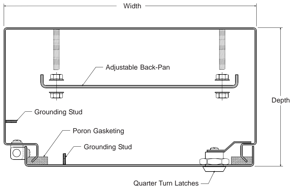
STANDARD ENCLOSURE SECTION VIEW
